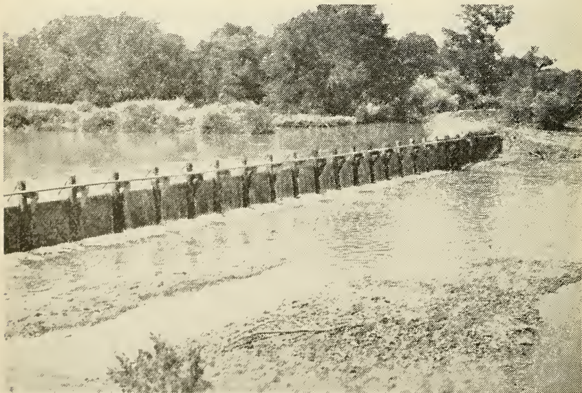
FIGURE 16. Moore Dam on Cache Creek. View from downstream side, showing Adams Canal coming into Cache Creek from north side. The water then crosses over and is taken out from the south side as the Moore Canal. June 18, 1940.
