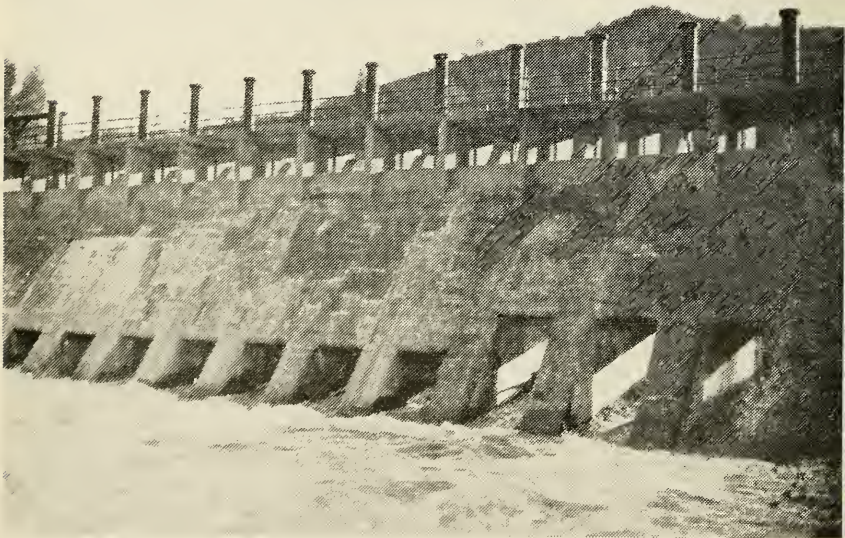
FIGURE 13. Clear Lake Impoundment Dam on Cache Creek. Outlet gates at bottom of dam are open. March 7, 1940
