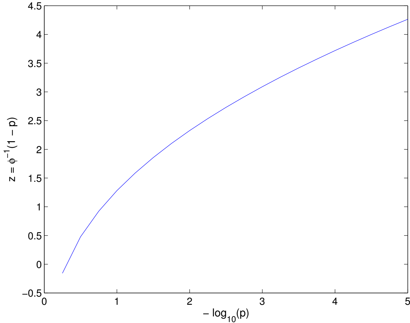
The relationship between logarithmically-spaced p-values and equivalent z
