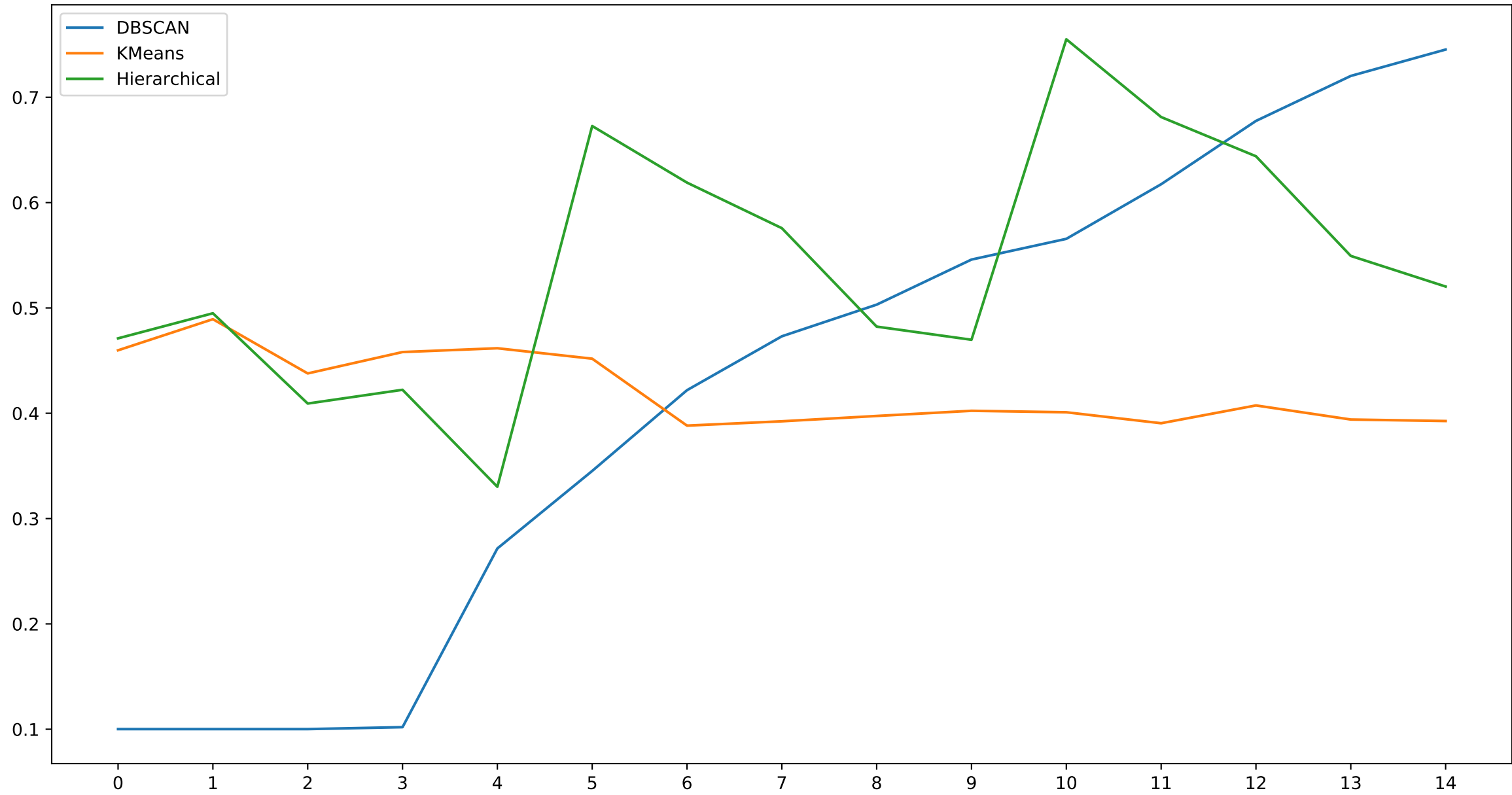
Silhouette score
